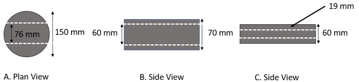
Figure 20. Trimming of samples for this study. A) Edge trimming- two cuts B) Surface trimming- two cuts C) Final trimming- three cuts
